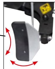
Adjustable bead breaker blade with protection and double acting cylinder
