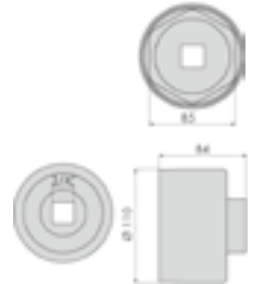
OM 0372 3/4" ROLLER BEARING AXLE NUT SOCKET BPW 16T HEX
